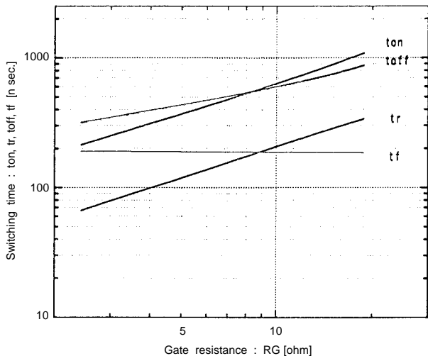
Switching time vs. RG Vcc=300V, Ic=200A, VGE=±15V, Tj=25°C
